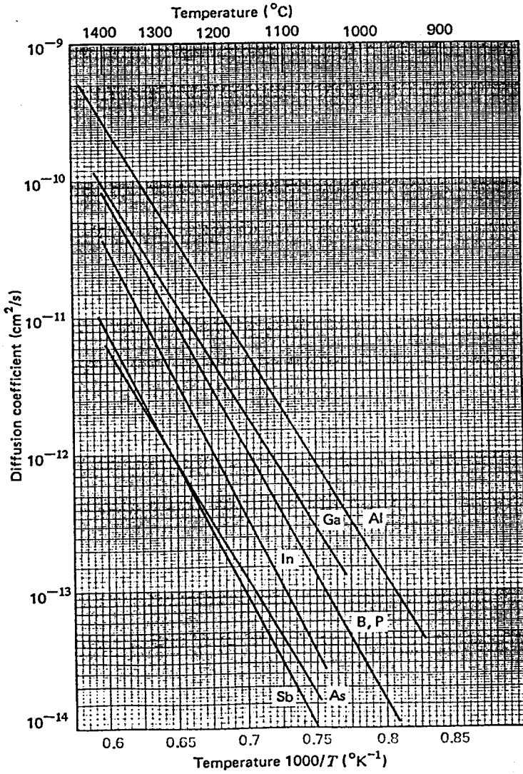
Fig. 4.7 Average diffusion coefficients for substitutional diffusers in silicon.
